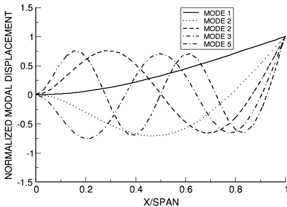
Fig. 2 Bending mode shapes of a fin.
