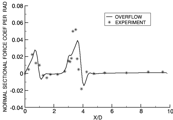
Fig. 5 Comparison of rate of normal sectional force coefficient with respect to AOA.
