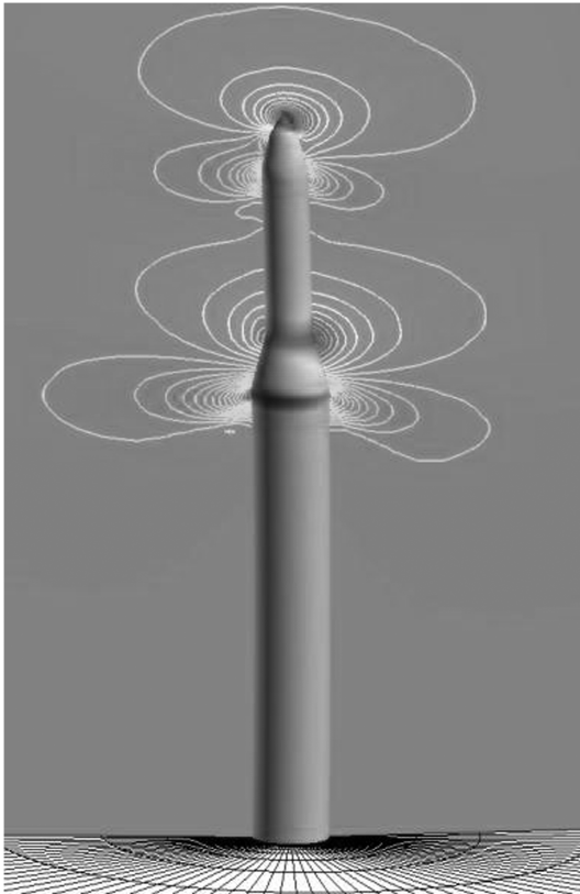
Fig. 10 Pressure distribution on deformed configuration.
