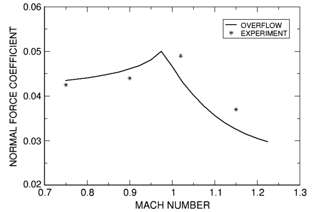
Fig. 7 Effect of Mach number on slope of normal force coefficient.
