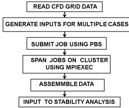
Fig. 1 RUNMAS parallel AIC computing approach.
