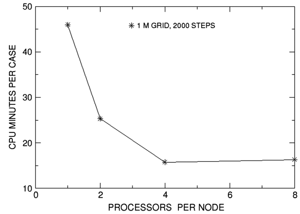
Fig. 12 Effect of OpenMP processors on computing time.
