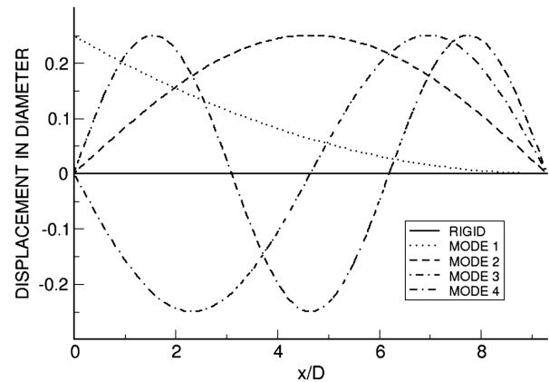
Fig. 9 First four modes of launch vehicle.
