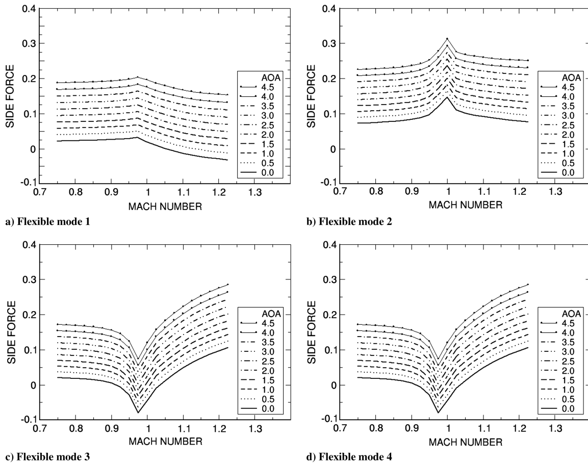
Fig. 15 Effect of Mach number and AOA on normal (side) force for four flexible modes.
