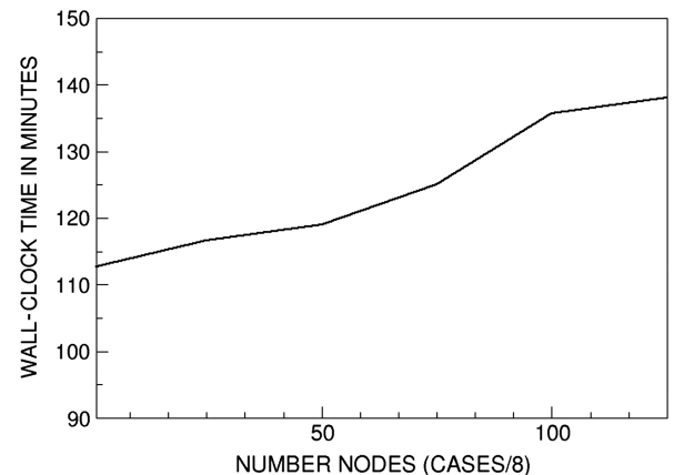
Fig. 13 Wall-clock time vs nodes.
