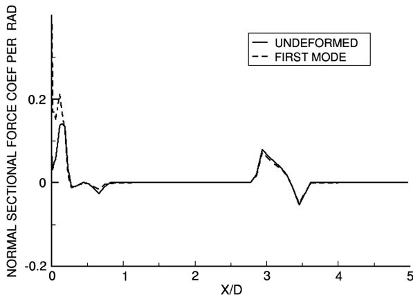
Fig. 11 Effect of first mode on normal sectional force coefficient.
