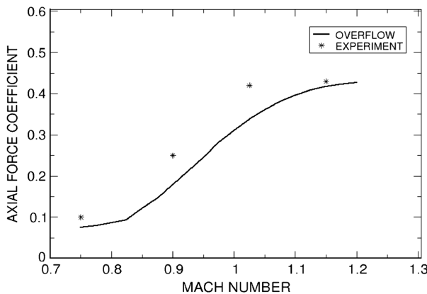
Fig. 6 Effect of Mach number on axial force coefficient.
