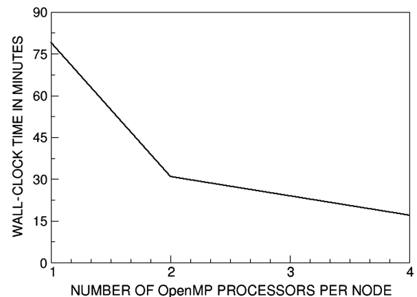
Fig. 14 Effect of OpenMP on wall-clock time.
