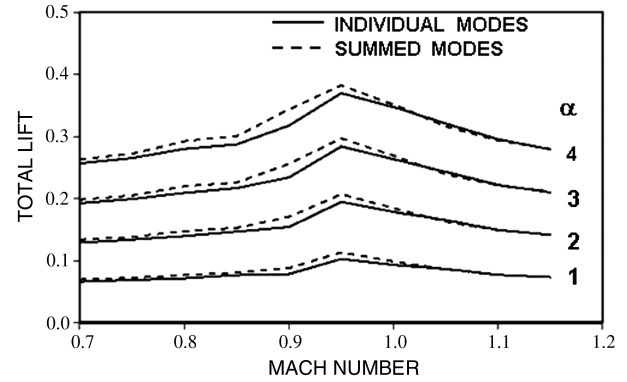
Fig. 3 Comparison lifts between individual modes and summed modes.
