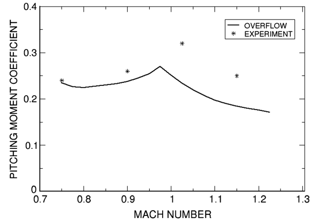
Fig. 8 Effect of Mach number of moment coefficient.
